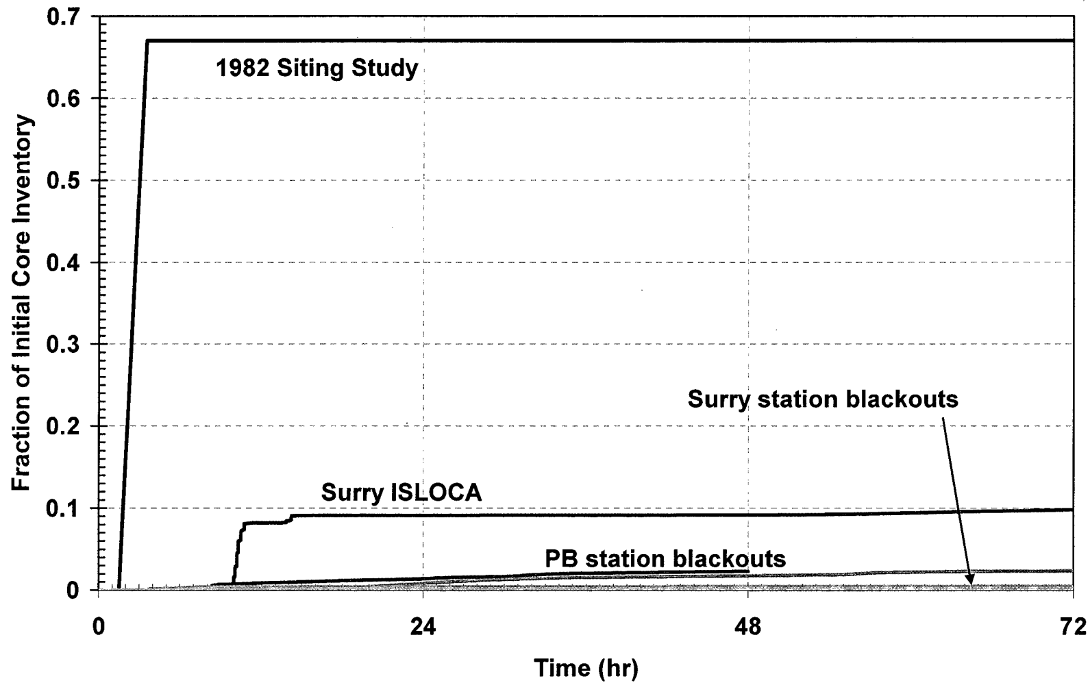
Cesium Release to the Environment for Unmitigated Cases
