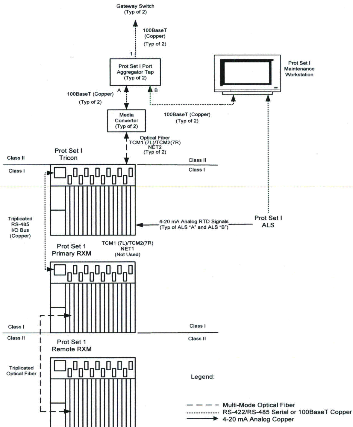
Figure 1: Tricon Protection Set and its Class II Communication.
