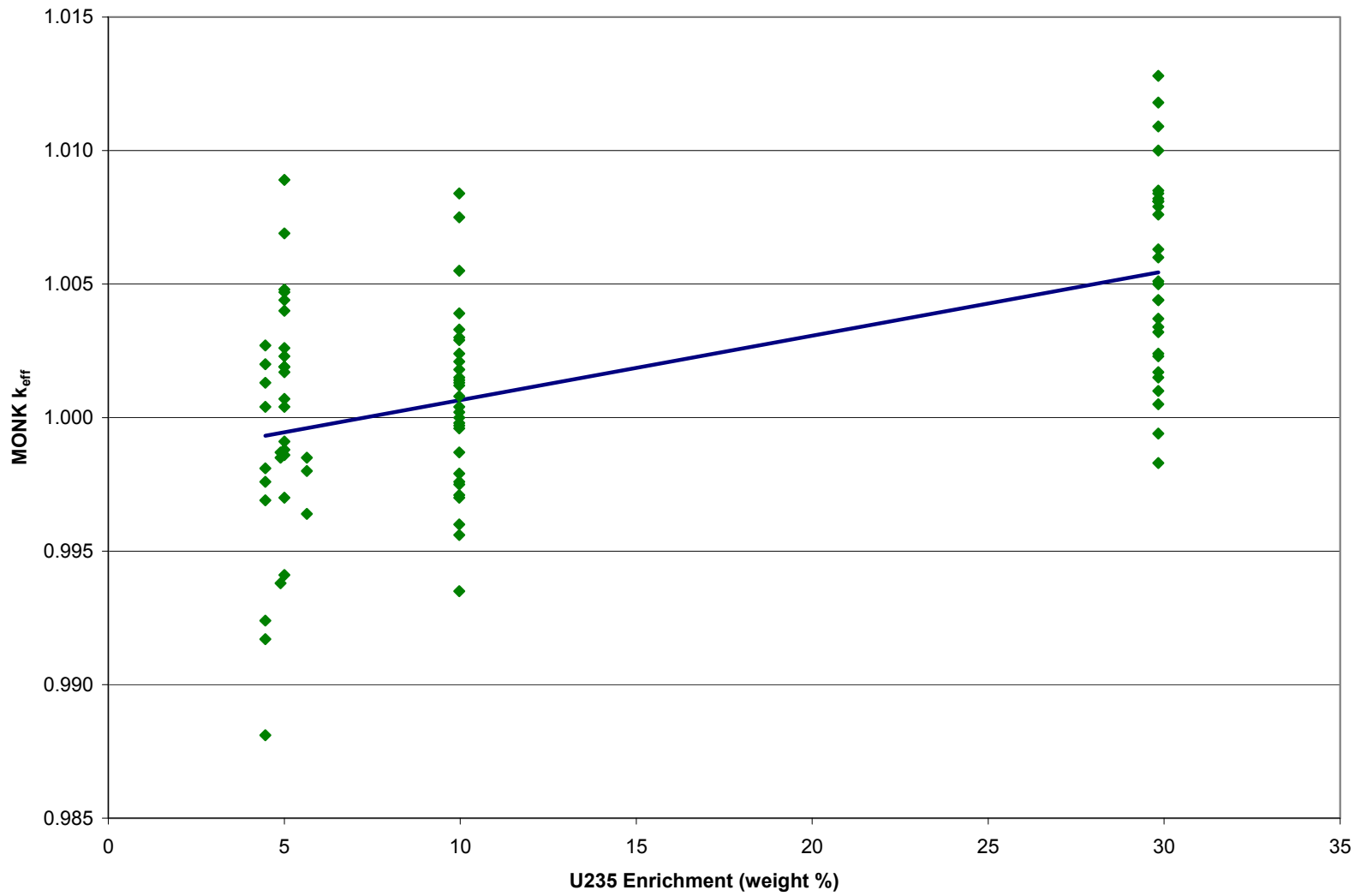
Figure 6-4: Plot of MONK8A k_{eff} vs. ^{235}\text{U} Enrichment
