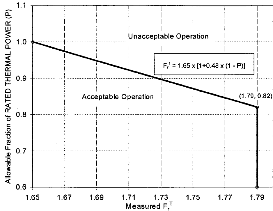
FIGURE 3.2-3 Allowable Combinations of THERMAL POWER and F_r^T
