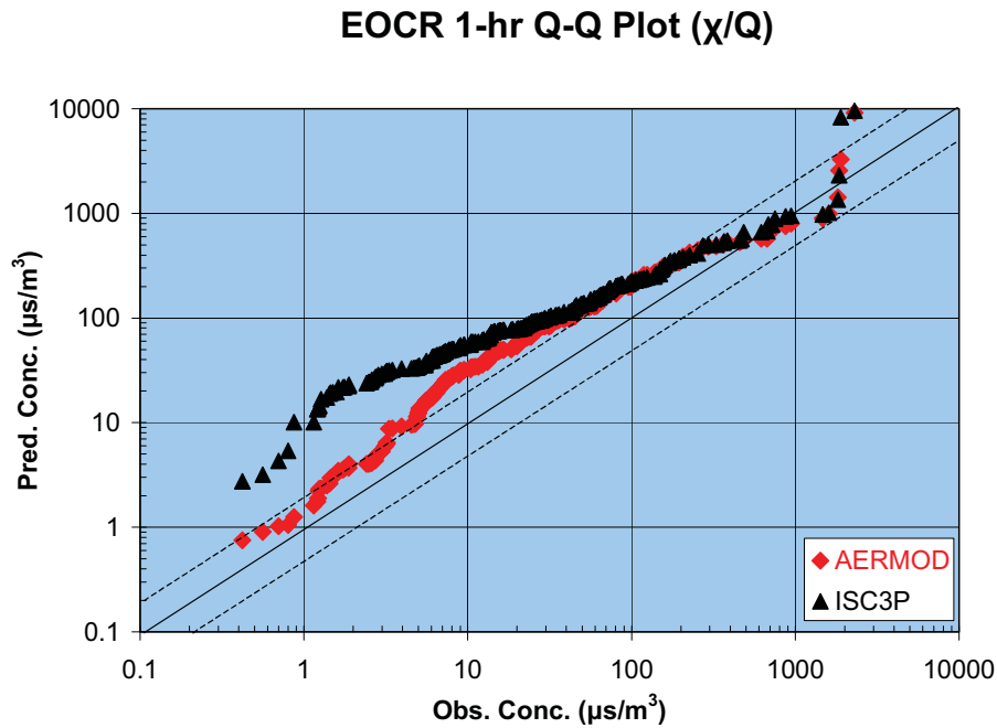
Figure 17. Q-Q Plot for EOGR 1-Hour Averages ( \text{SF}_6 )
