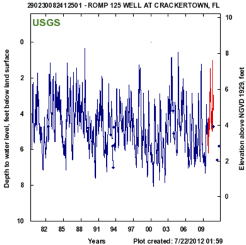
Monitoring Well Water Level Elevation Above NVGD 1929 (Seawater Reference Level)
