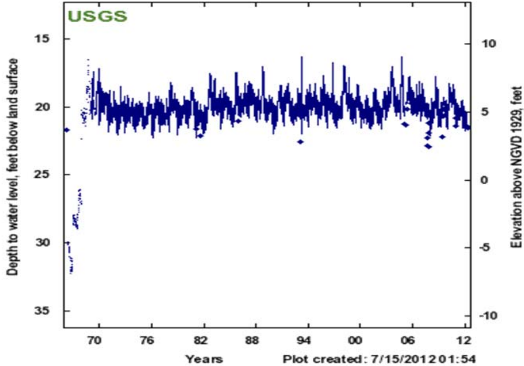
Monitoring Well Water Level Elevation Above NVGD 1929 (Seawater Reference Level)
