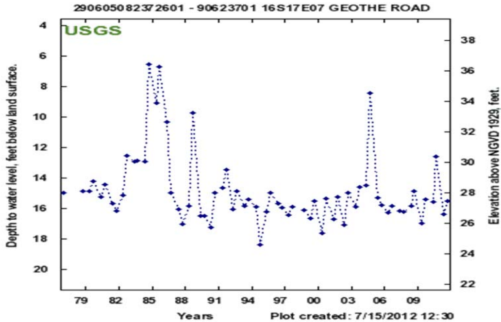
Monitoring Well Water Level Elevation Above NVGD 1929 (Seawater Reference Level)
