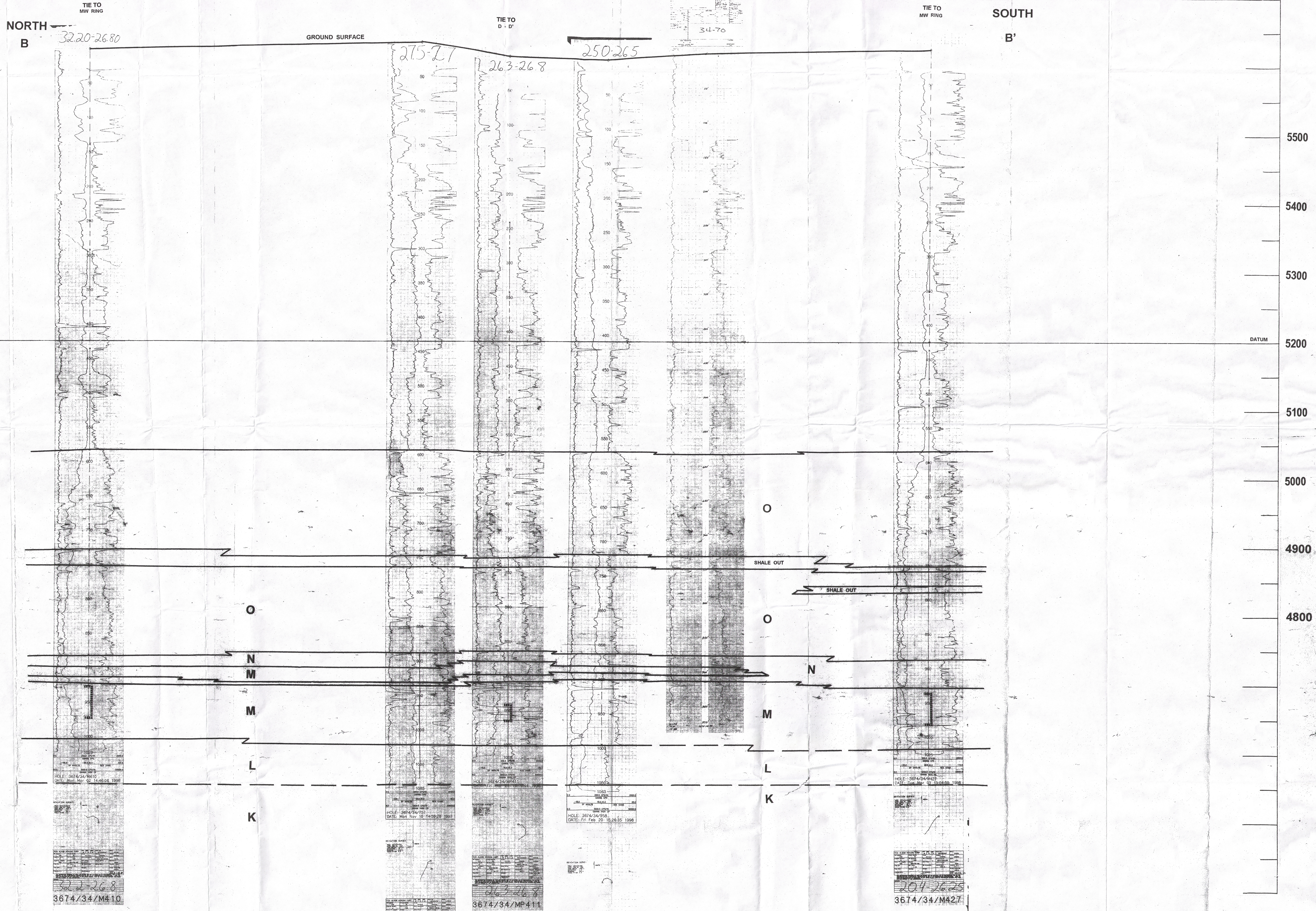
RIO ALGOM MINING SMITH RANCH PROJECT FIGURE D-5.19 GEOLOGIC CROSS-SECTION B - B' LOOKING EAST
