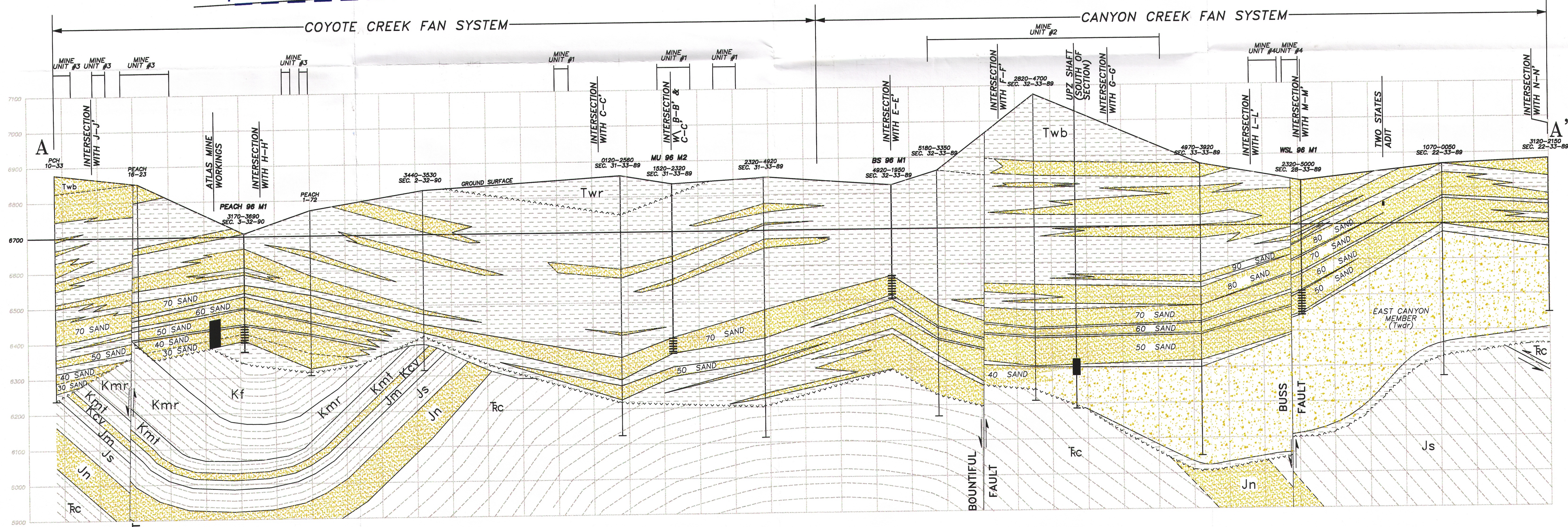
CROSS SECTION A-A' SCALE: 1" = 2000' HORIZONTAL 1" = 200' VERTICAL
