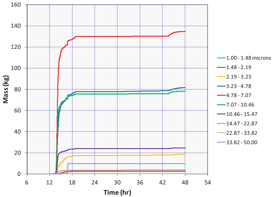
Figure 4-21 Masses of Radionuclides Sourced into the ISLOCA Deposition Calculation by Size
