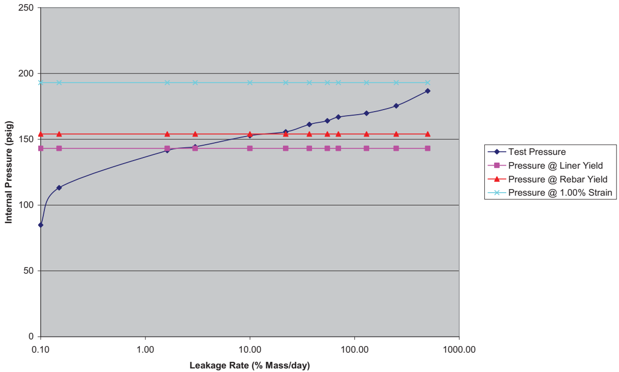
1:4 Scale Prestressed Concrete Containment Test Pressure Vs. Leakage Rate
