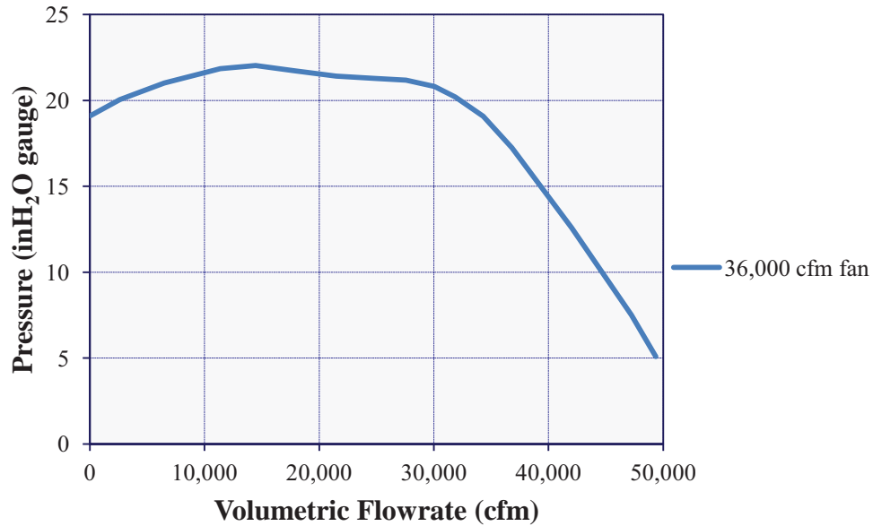
Figure D-4 Auxiliary Ventilation System Safety-Related Fan Curve
