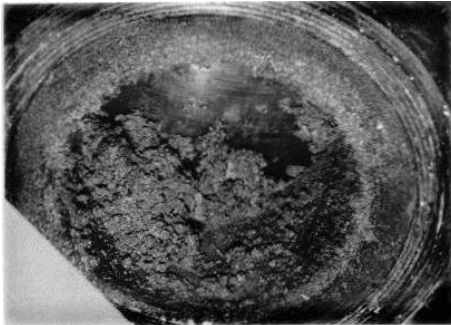
Figure D-6 Test LA3C, Downstream end of pipe 6 showing large deposit
