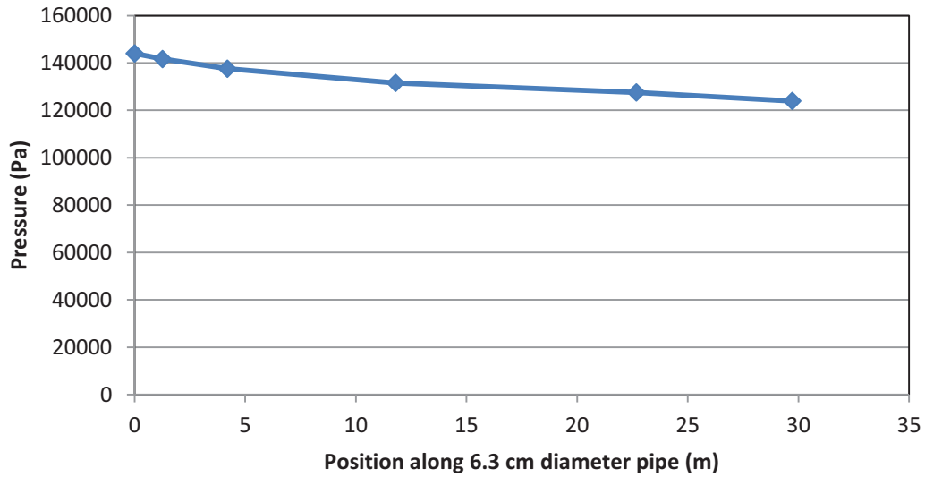
Figure D-53 Pressure profile along test pipe
