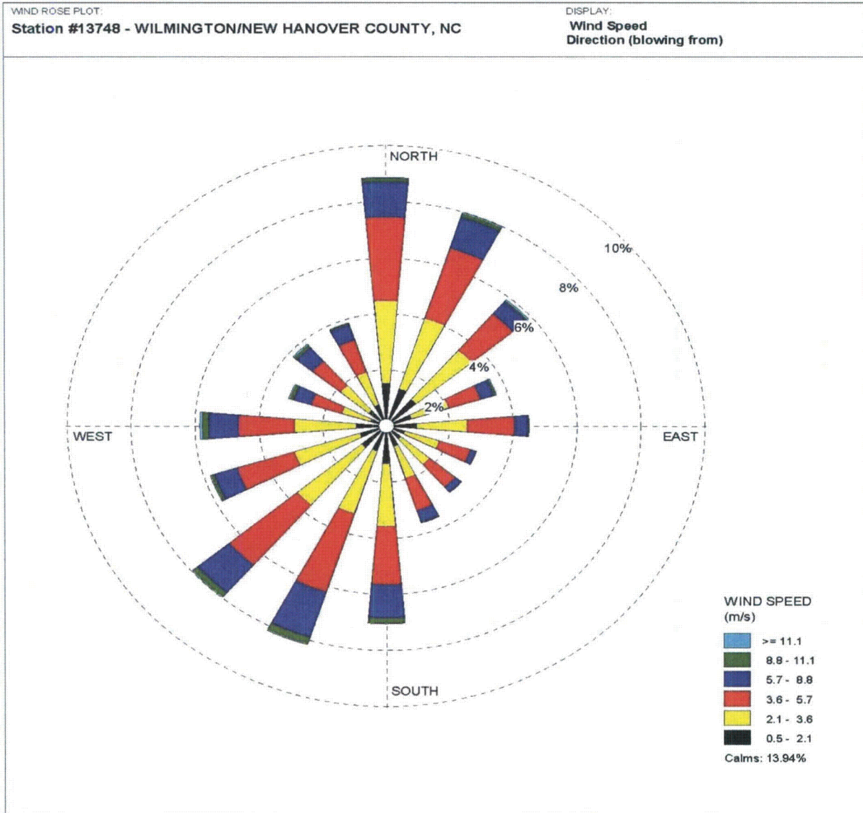
Figure 1-7. Wind Rose for Wilmington International Airport.
