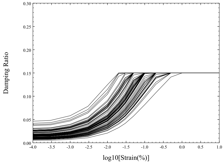
FIRS4 randomization - Damping curve 17
