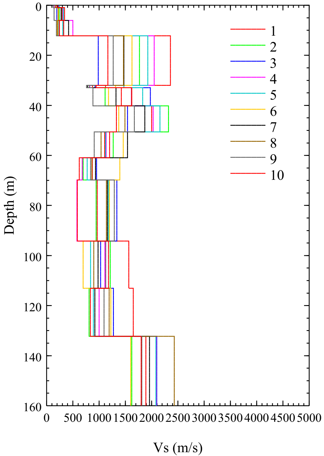
Figure 2.5.2-242 Graph of Velocity vs. Depth for the First 10 Synthetic Profiles Generated for the Top Portion of the FIRS4 Site Column
