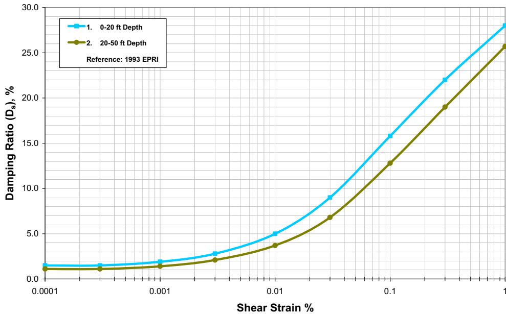
Figure 1b: Damping in Shear vs. Strain (Sand Characteristic Behaviour, EPRI 1993)
