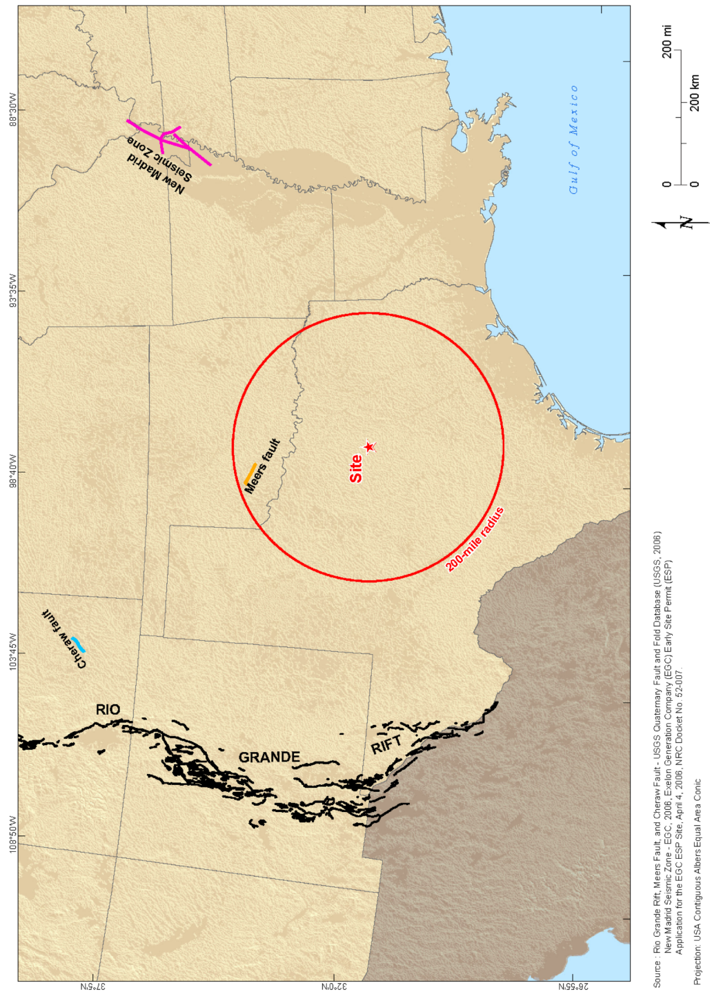
Figure 2.5.1-213 Significant Quaternary Features Outside of the Site Region
