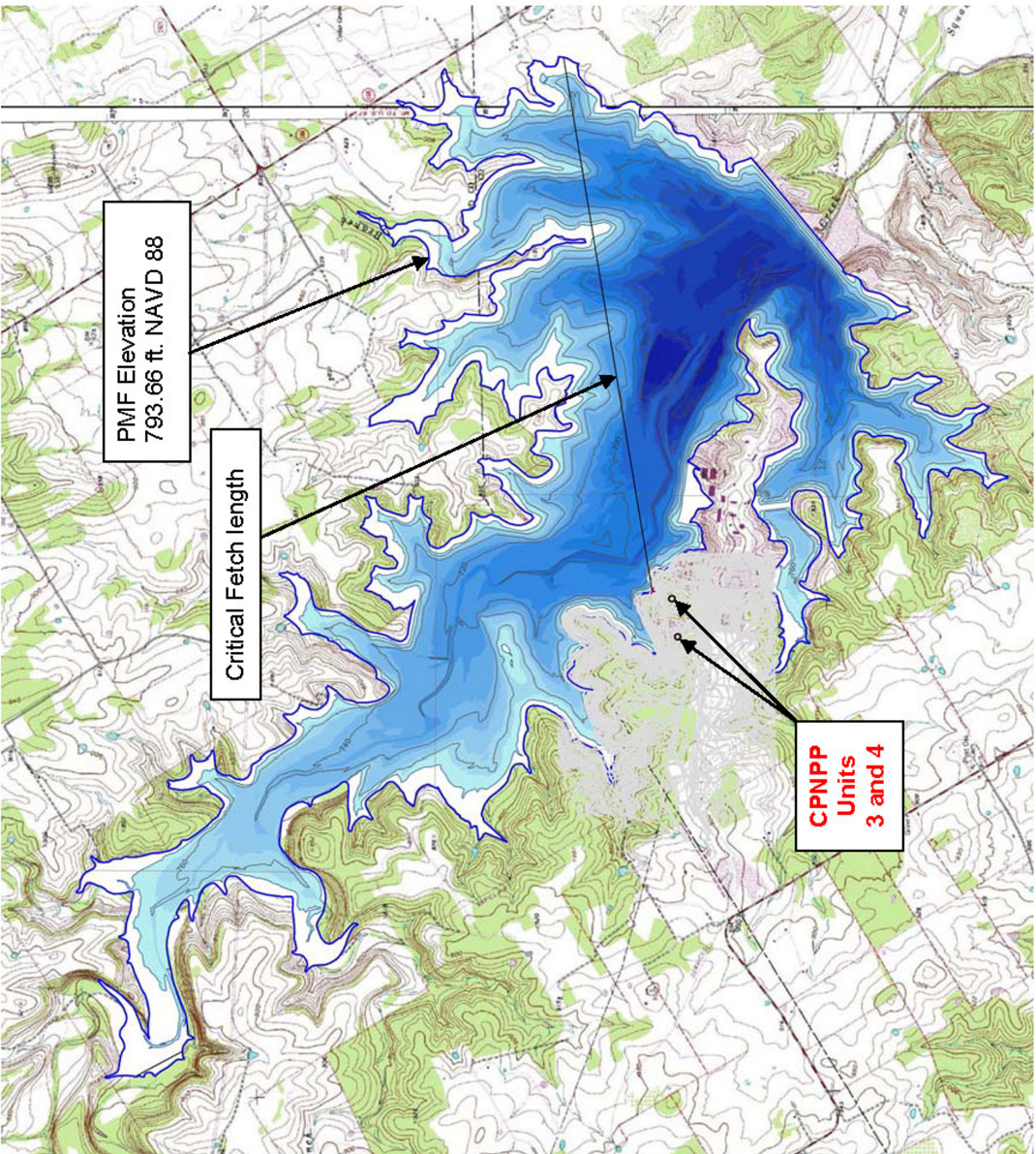
Figure 2.4.3-209 Coincident Wind Wave Activity Fetch Length
