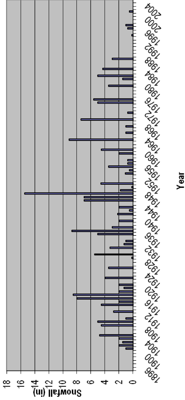
Weatherford Snowfall (1896-2005)
