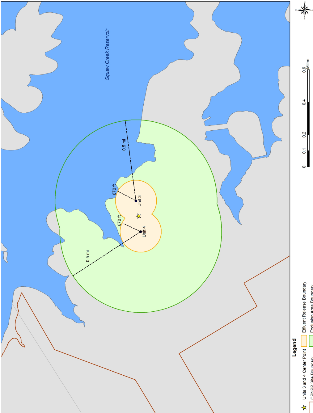
Figure 2.1-205 Distance to the Exclusion Area Boundary (EAB)
