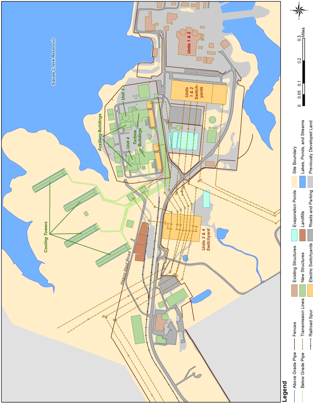
Figure 2.1-201 Site Plot Plan
