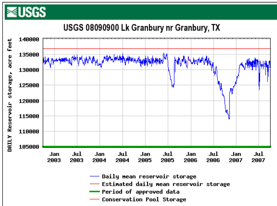
Figure 2.3-23 Lake Granbury Elevation and Storage Data (October 2002 to September 2007)
