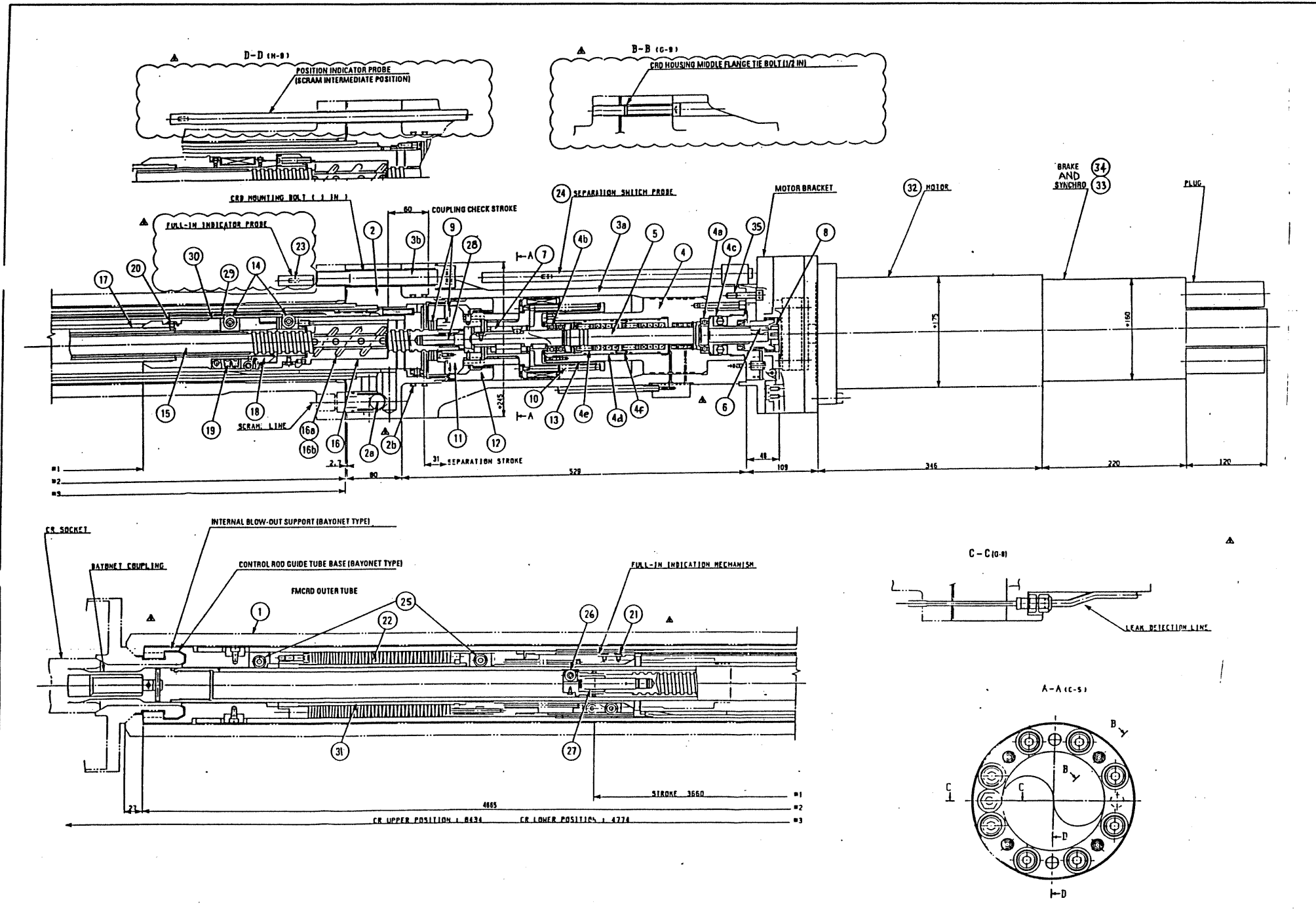
Figure 15B-3 Fine Motion Control Rod Drive
