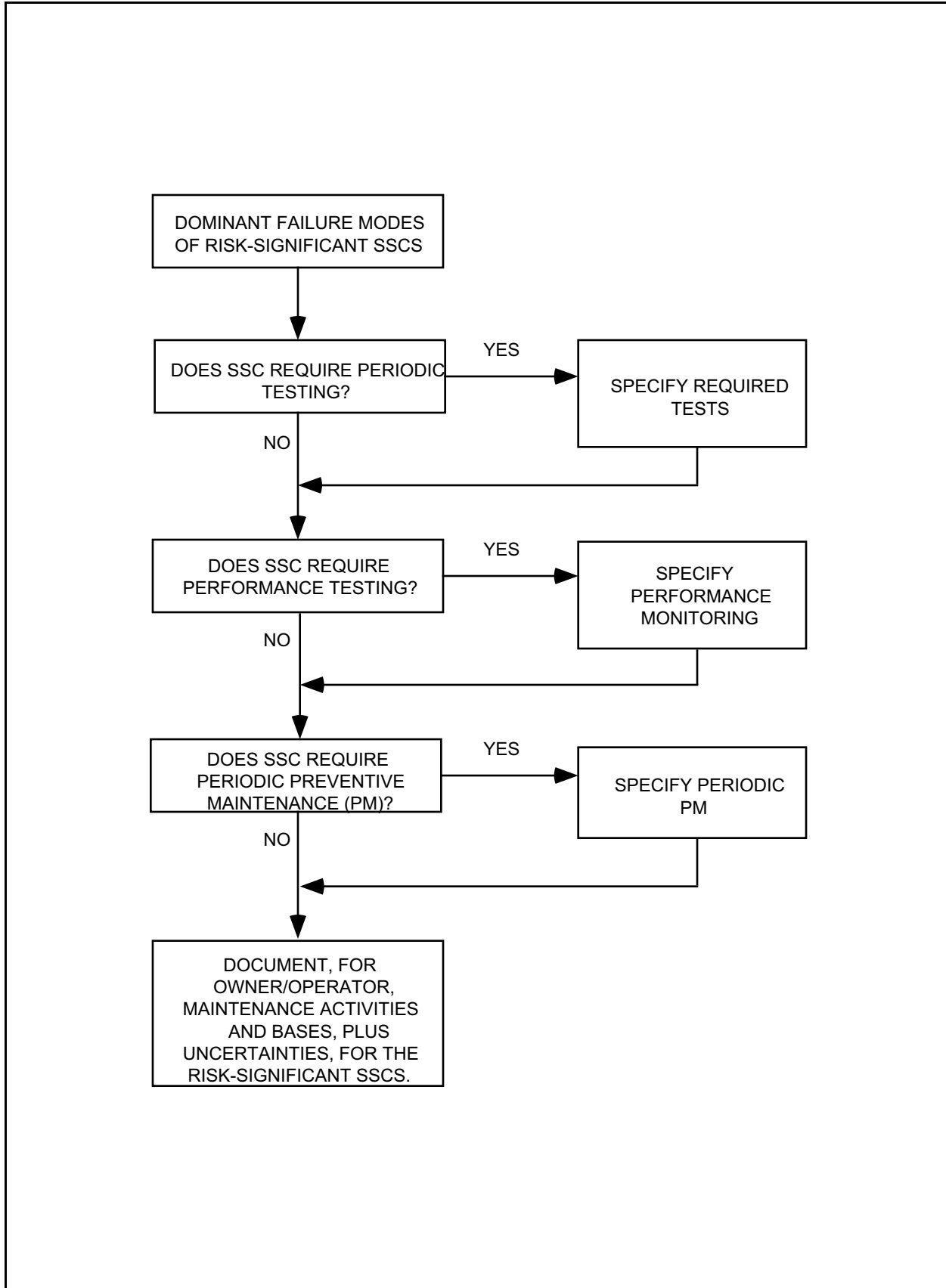
Figure 17.3-6 Identification of Risk-Significant SSC O-RAP Activities
