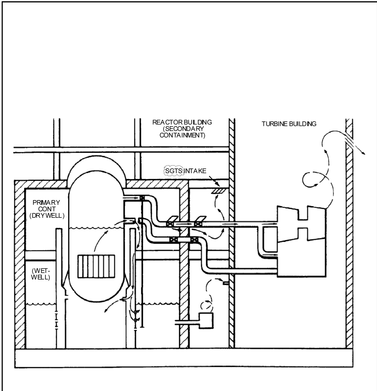
Figure 15.6-2 LOCA Radiological Analysis
