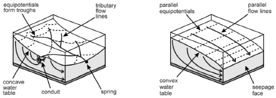
Figure 2. Carbonate/Karst Aquifer (left) versus an Porous Medium (right)
