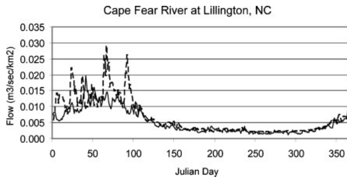
Figure 10. Example of Northern River Pattern (NRP) on the Cape Fear River in North Carolina (1000 km north of Florida) comparing median daily flows for two multidecadal time periods (1940–1969 (solid line) and 1970–1999 (bold broken line)). Flows are standardized per square kilometre of catchment area
