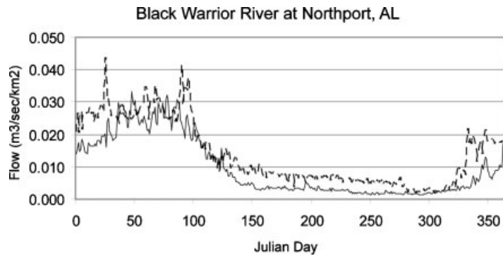
Figure 9. Example of Northern River Pattern (NRP) on the Black Warrior River in Alabama (northeast of Florida) comparing median daily flows for two multidecadal time periods (1940–1969 (solid line) and 1970–1999 (bold broken line)). Flows are standardized per square kilometre of catchment area
