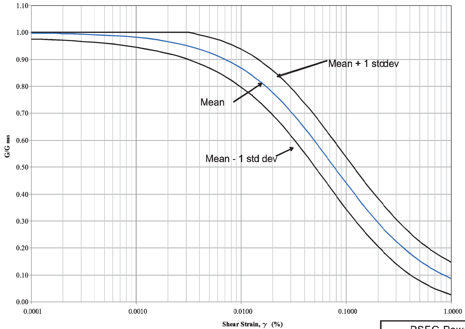
PSEG Power, LLC PSEG SITE ESPA Part 2, Site Safety Analysis Report Computed Modulus Reduction Curve Layer D FIGURE 2.5.4.7-27 Rev 0
