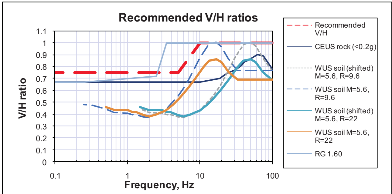
V/H ratios for CEUS rock, WUS soil (for M 5.6 and two distances), for WUS soil with frequency shifted (for M5.6 and two distances), and recommended V/H ratio. Distances, R, are in km. Equivalent distances in miles are: 9.6 km (6 mi); 22 km (13.7 mi).
