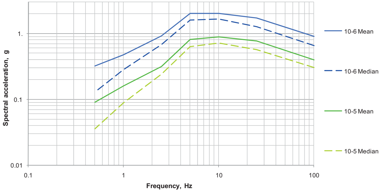
Soil UHRS for 10 -5 and 10 -6 , Mean and Median for PSEG site
