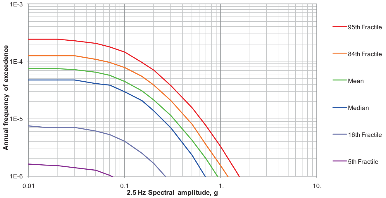
2.5 Hz Soil Seismic Hazard Curves
