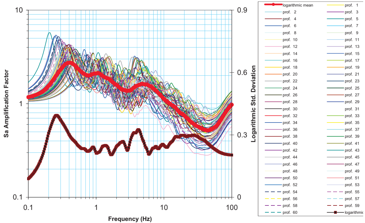
Amplification Factors (Left Y Axis) and Associated Logarithmic Standard Deviation (Right Y Axis) Calculated with the 60 Synthetic Profiles, for the 10-5 Low-Frequency Rock Input
