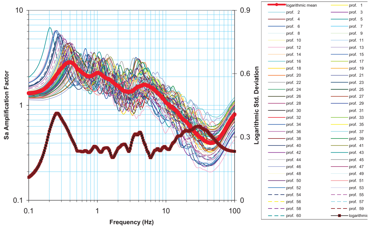
Amplification Factors (Left Y Axis) and Associated Logarithmic Standard Deviation (Right Y Axis) Calculated with the 60 Synthetic Profiles, for the 10-5 High-Frequency Rock Input
