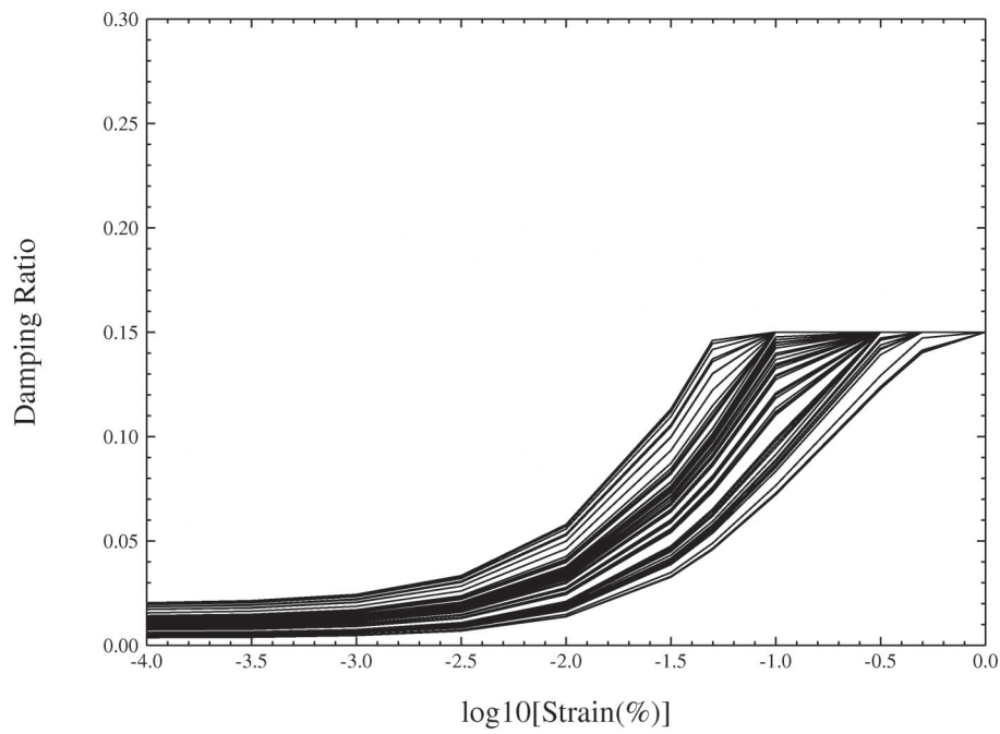
Damping curve 02 (Layers 2-5)
