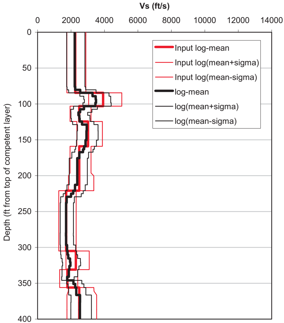
Comparison of Input Values of Logarithmic Mean \pm Sigma of Shearwave Velocity to Values Calculated from the 60 Synthetic Profiles (Shallow Portion)
