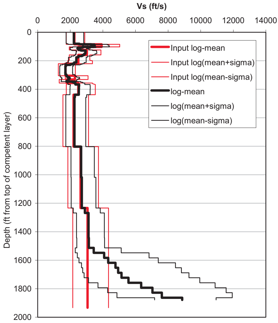
Comparison of Input Values of Logarithmic Mean \pm Sigma of Shearwave Velocity to Values Calculated from the 60 Synthetic Profiles
