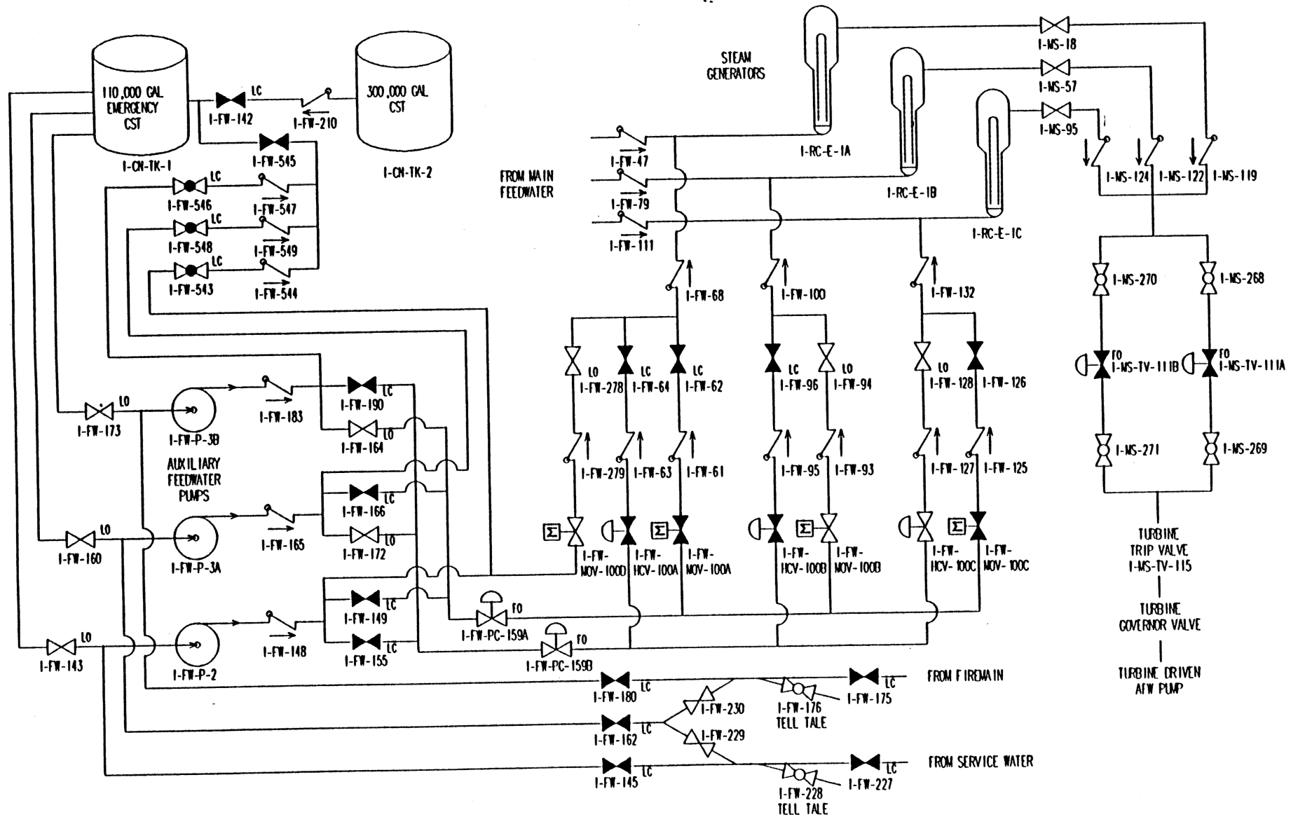
FIGURE A.13-1 AUXILIARY FEEDWATER SYSTEM
