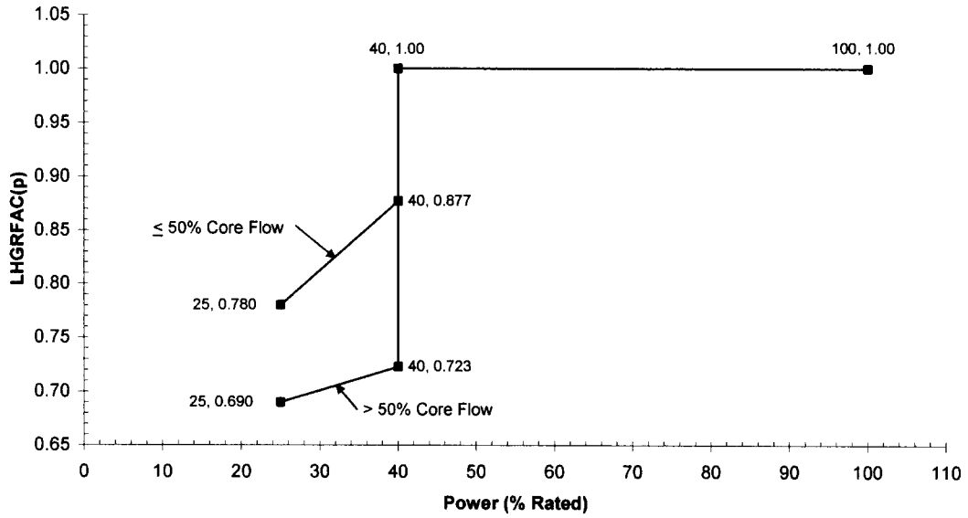
Figure 3-1a Cycle 19 Power-Dependent LHGR Factor BOC-MOC for GNF2 and GE14 Note: These factors to be applied to the exposure-dependent limits as described in Section 5.3
