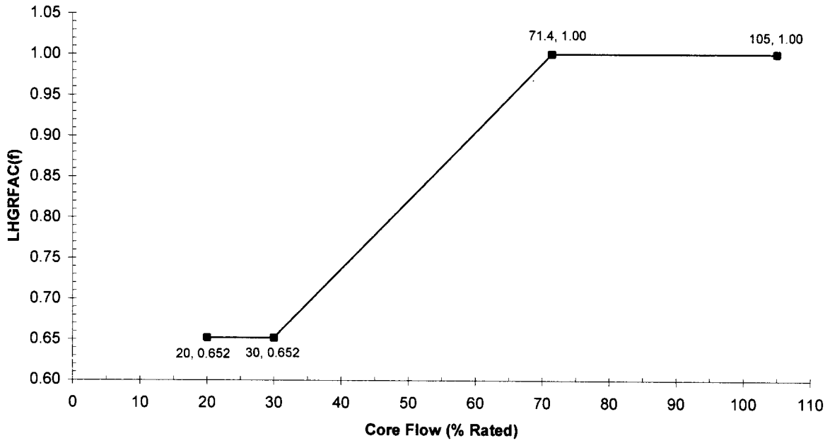
Figure 3-2 Cycle 19 Flow-Dependent LHGR Factor for GNF2 and GE14 Note: These factors to be applied to the exposure-dependent limits as described in Section 5.3
