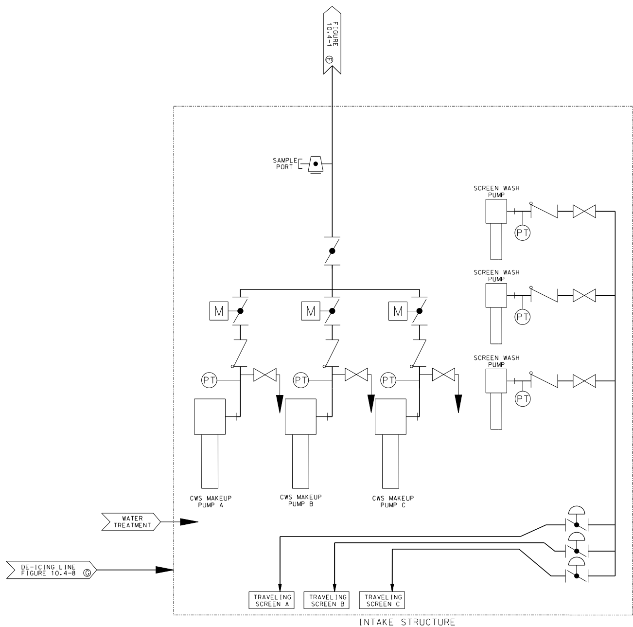
Figure 10.4-6— {Circulating Water System P&ID (Makeup System)}
