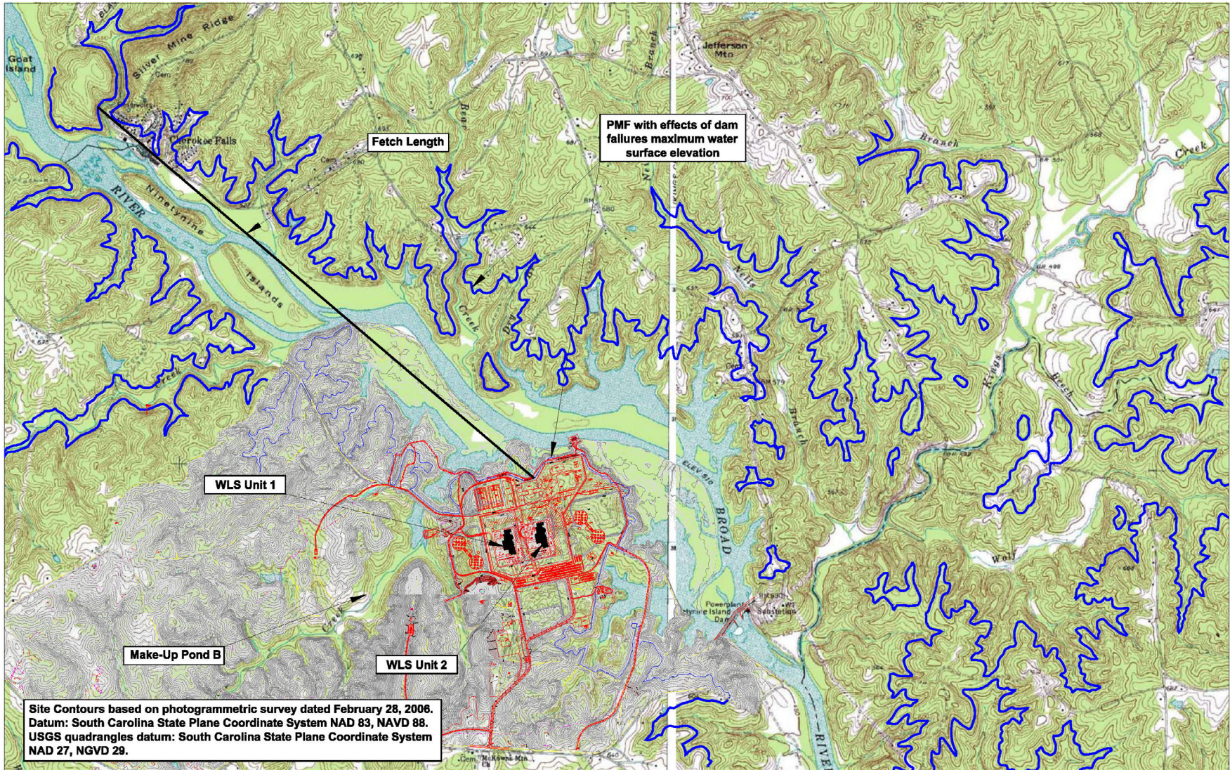
WILLIAM STATES LEE III NUCLEAR STATION UNITS 1 & 2 Broad River Coincident Wind Wave Fetch Length FIGURE 2.4.4-201 Rev 5
