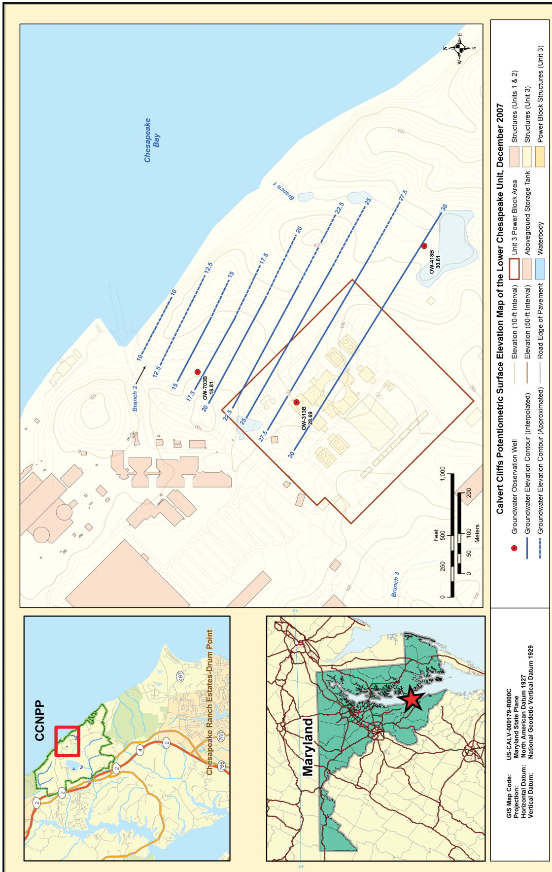
Figure 2.3-90— Potentiometric Surface Elevation Map for the Lower Chesapeake Unit, December 2007
