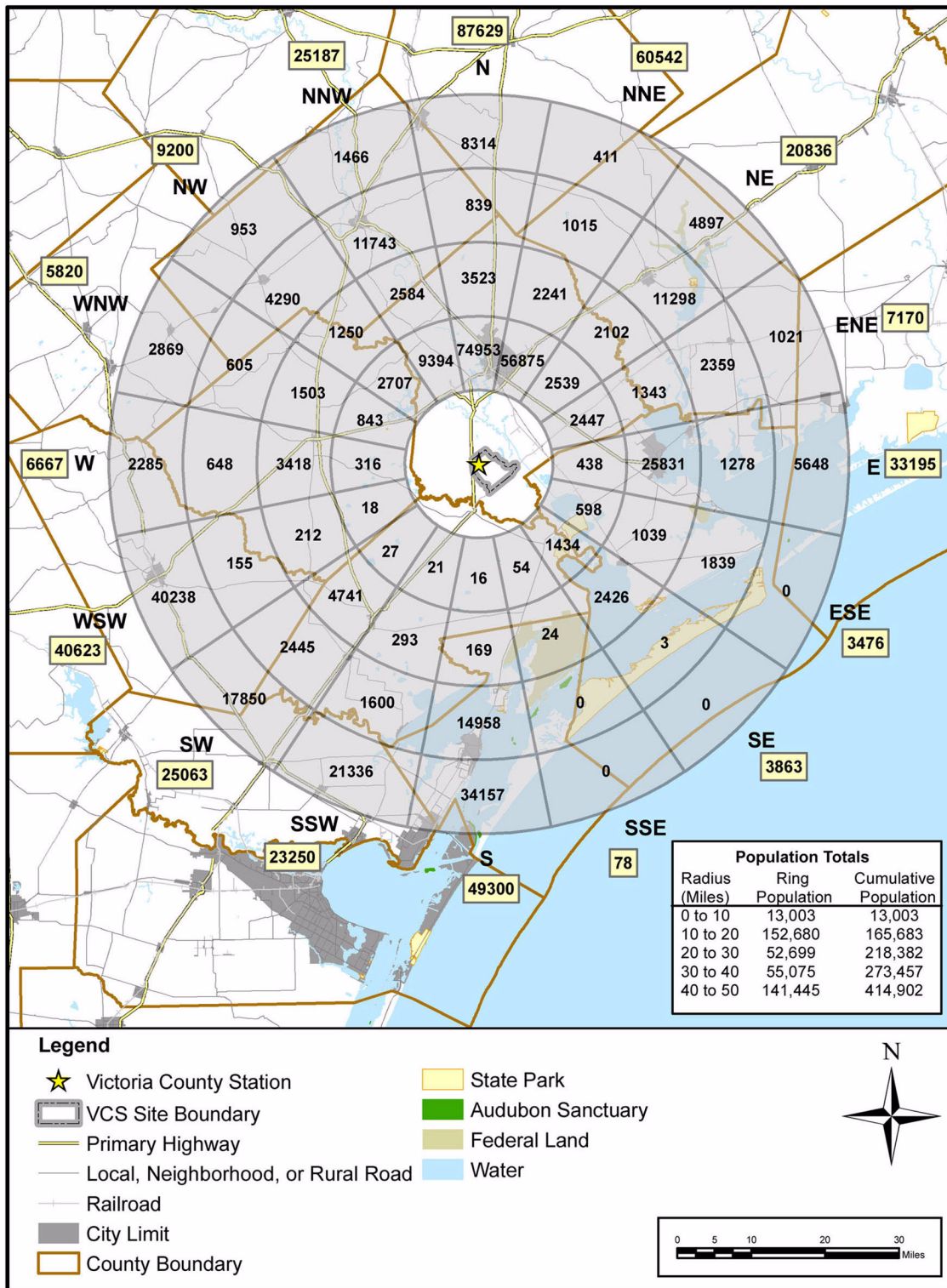
Figure 2.1-25 10- to 50-Mile 2080 Population Distribution
