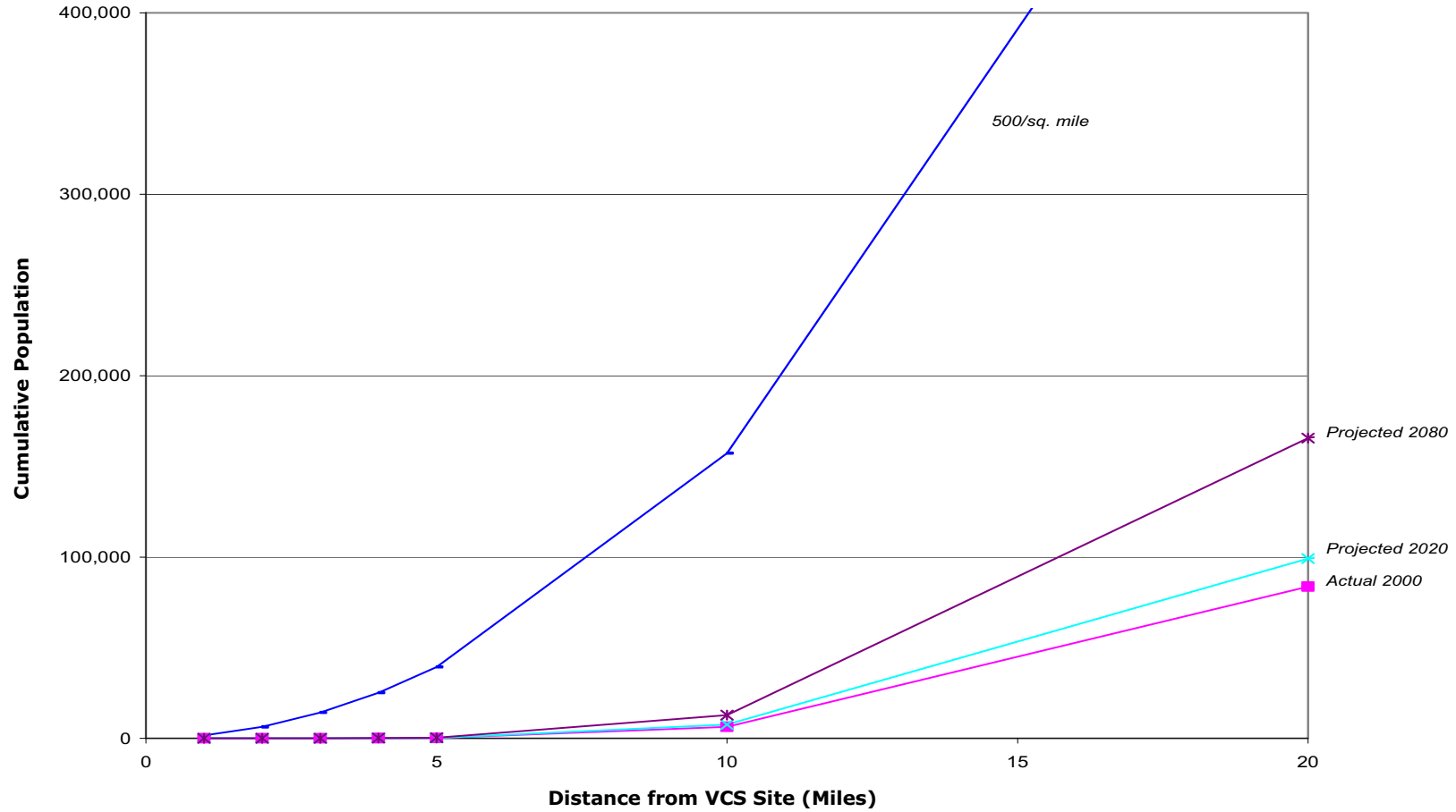
Figure 2.1-28 Population Compared to NRC Siting Criteria
