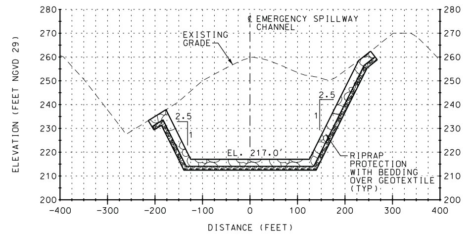
SECTION B NOTE: SEE PLAN FOR CROSS SECTION LOCATION
