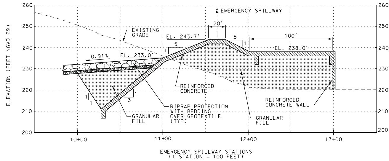
SECTION A NOTE: SEE PLAN FOR CROSS SECTION LOCATION
