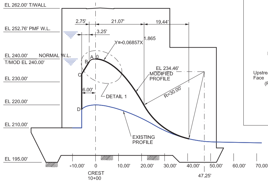
SECTION A MODIFIED SPILLWAY PROFILE (PRELIMINARY)
