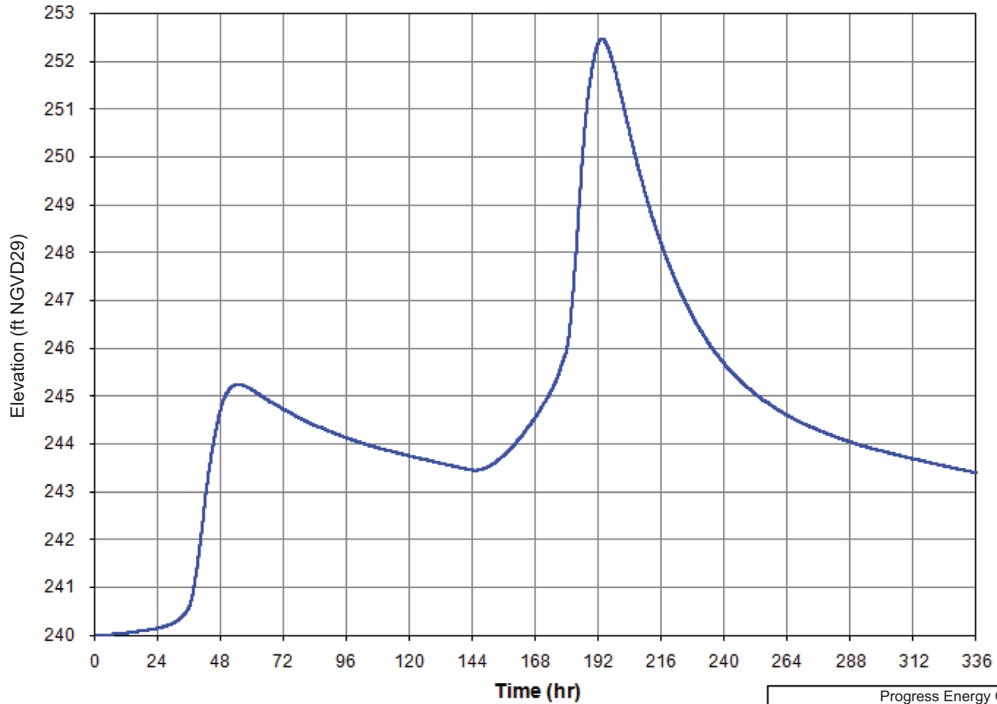
Progress Energy Carolinas Shearon Harris Nuclear Power Plant Units 2 and 3 Part 2, Final Safety Analysis Report New Hill, North Carolina PMF Stillwater Elevation in the Main Reservoir FIGURE 2.4.3-225 Rev 4
