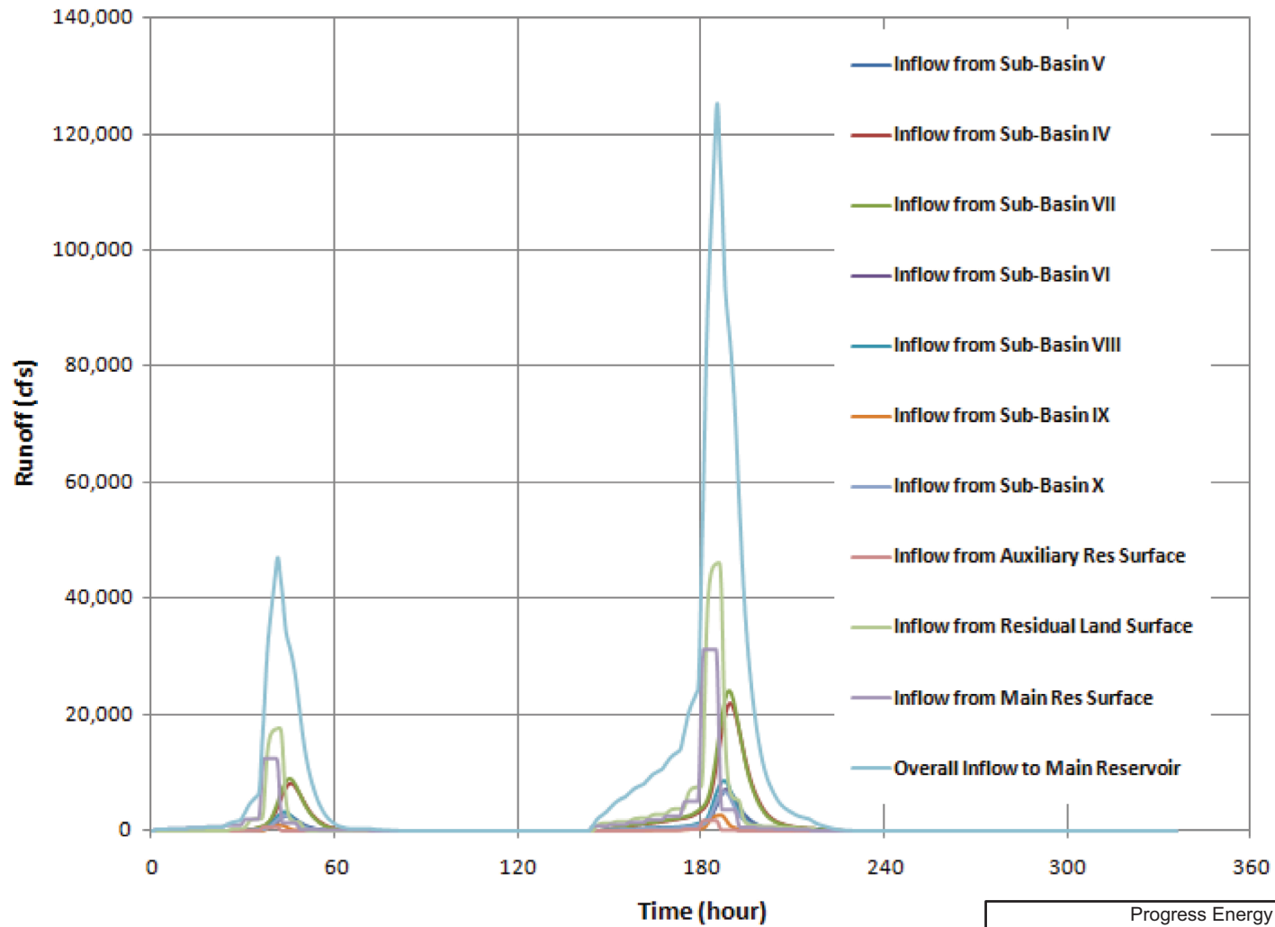
Progress Energy Carolinas Shearon Harris Nuclear Power Plant Units 2 and 3 Part 2, Final Safety Analysis Report New Hill, North Carolina Unsteady Flow Data, Boundary Condition of the HEC-RAS Model FIGURE 2.4.3-221 Rev 4
