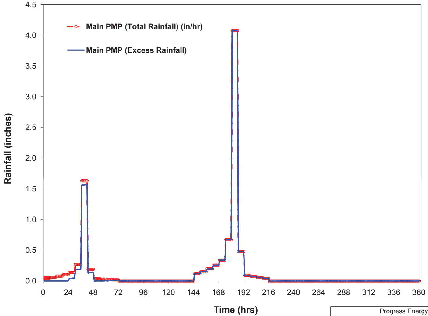
Progress Energy Carolinas Shearon Harris Nuclear Power Plant Units 2 and 3 Part 2, Final Safety Analysis Report New Hill, North Carolina Actual and Effective Precipitation for Main Drainage Basin FIGURE 2.4.3-210
