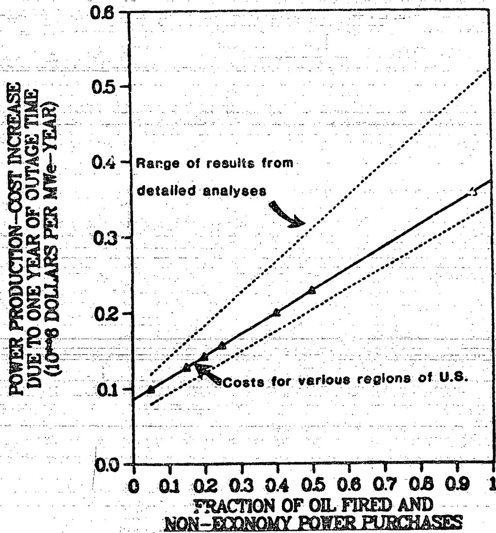
Figure 3.1 - Relationship between power production cost increase and non-economy power fraction [E.C.].
