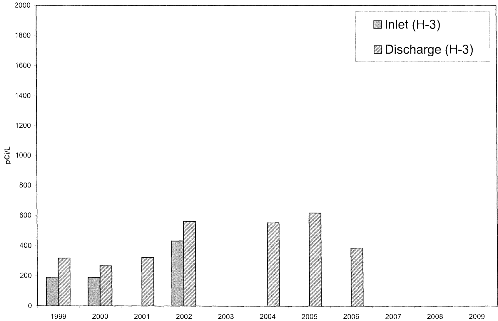
FIGURE C-3 RADIONUCLIDES IN HUDSON RIVER WATER 1999 to 2009
