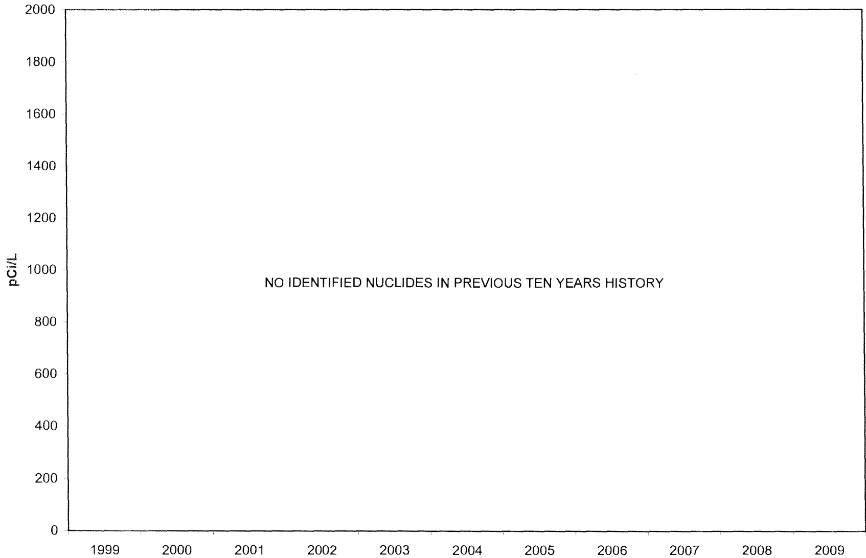
FIGURE C-4 RADIONUCLIDES IN DRINKING WATER 1999 to 2009
