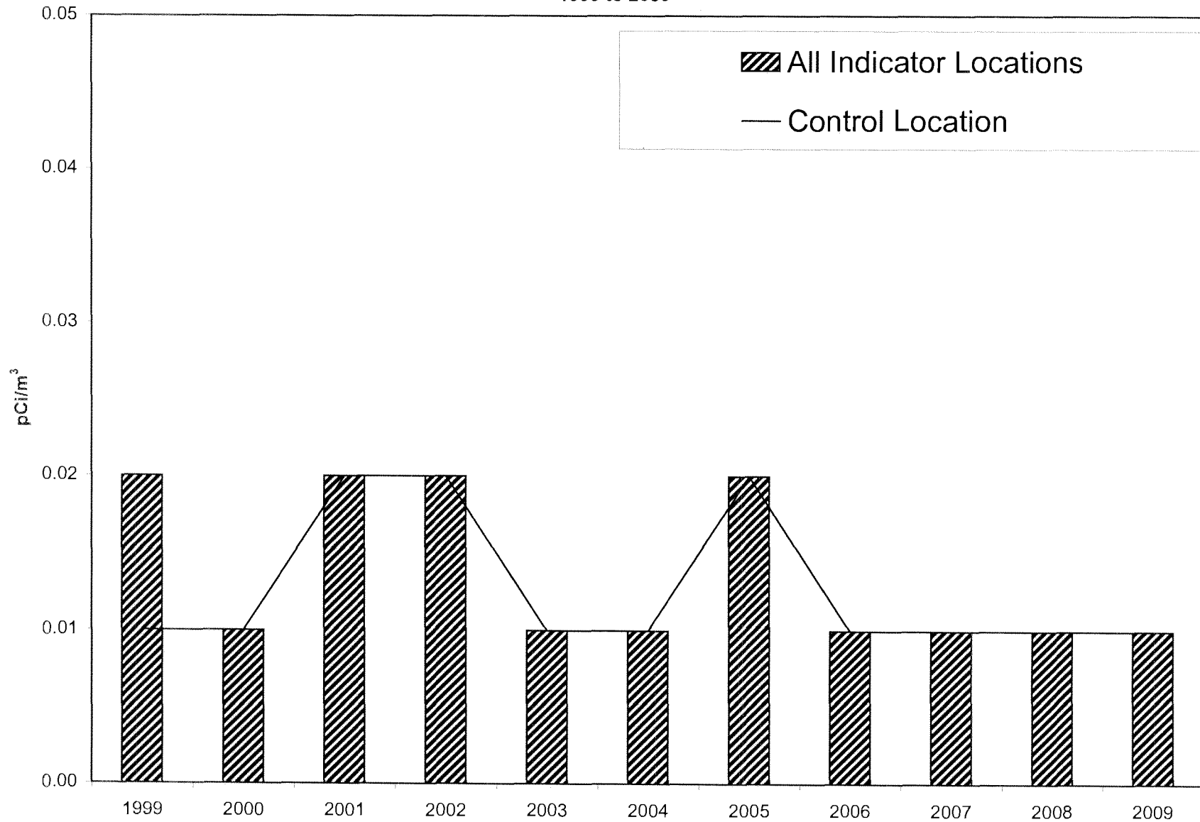
FIGURE C-2 RADIONUCLIDES IN AIR - GROSS BETA 1999 to 2009
