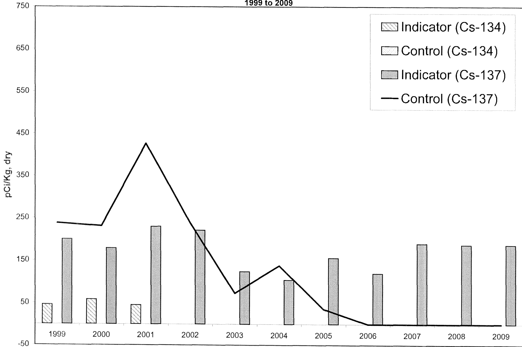
FIGURE C-5 RADIONUCLIDES IN SHORELINE SOIL 1999 to 2009
