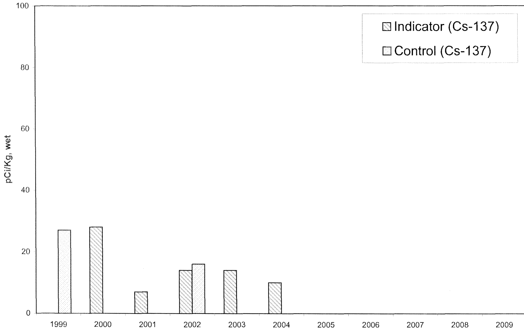
FIGURE C-6 BROAD LEAF VEGETATION - Cs-137 1999 to 2009
