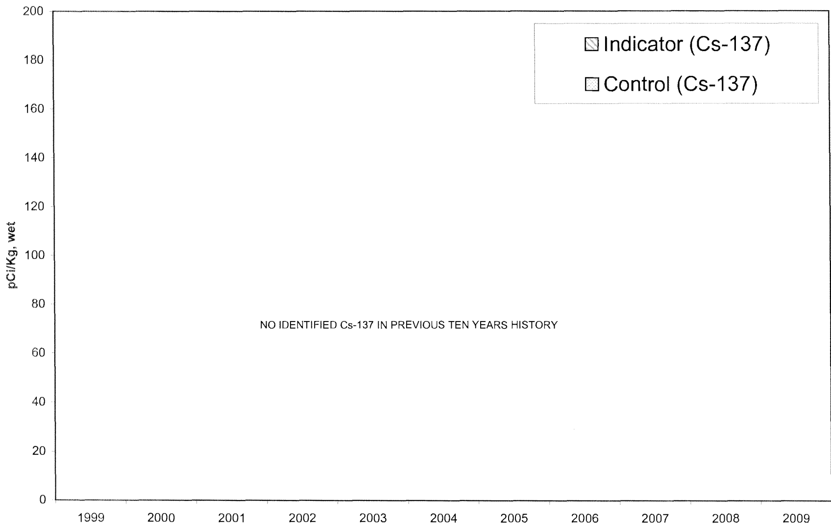
FIGURE C-7 FISH AND INVERTEBRATES - Cs-137 1999 to 2009
