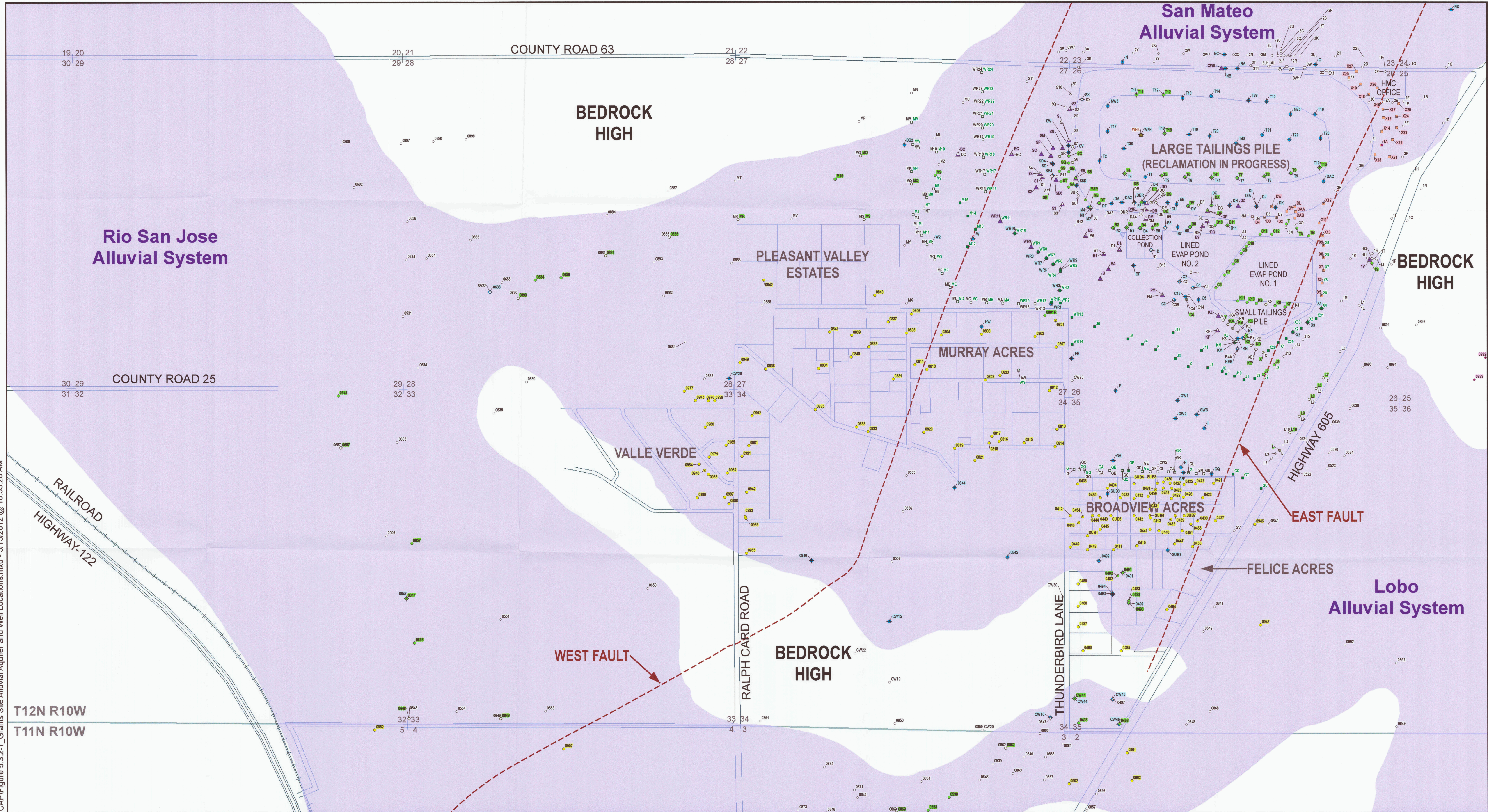
GRANTS RECLAMATION PROJECT Updated Corrective Action Program (CAP) FIGURE 5.3.2-1 GRANTS SITE ALLUVIAL AQUIFER AND WELL LOCATIONS
