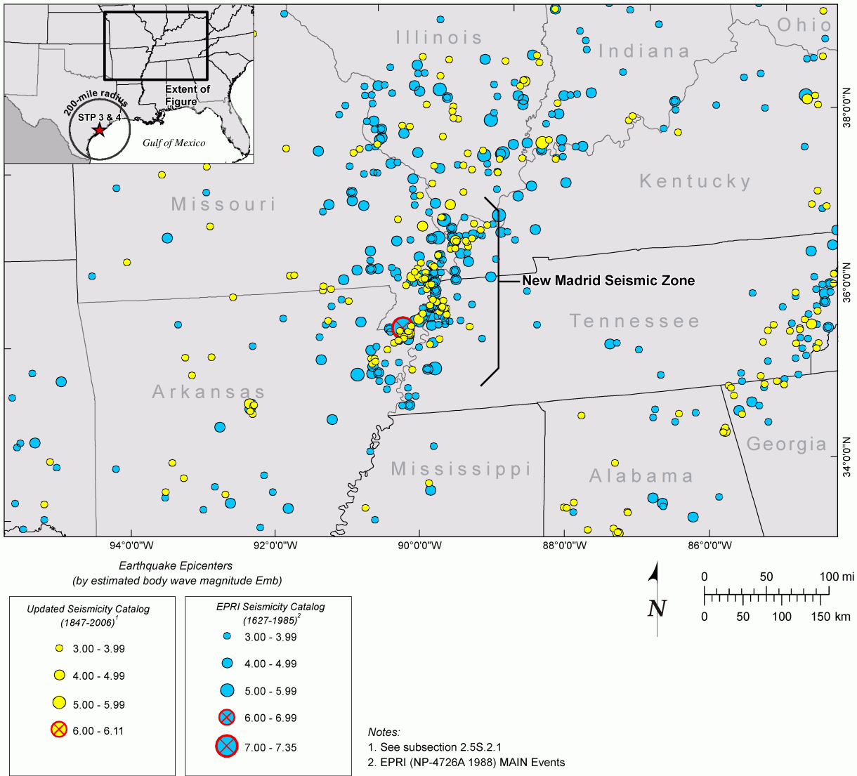
Figure 2.5S.2-9 New Madrid Seismic Zone Seismicity
